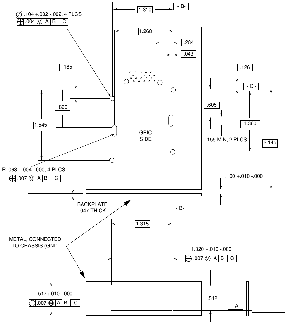
Figure 12: Typical Host Card Footprint
